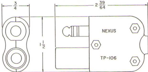
TP-106 TELEPHONE PLUG BIAxIAL SHIELDED SIX CONDUCTOR
