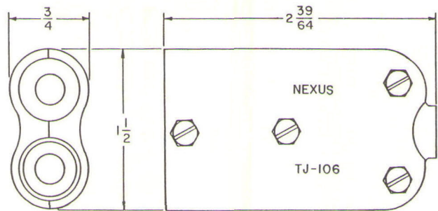
TJ-106 TELEPHONE JACK BIAxIAL SHIELDED SIX CONDUCTOR
